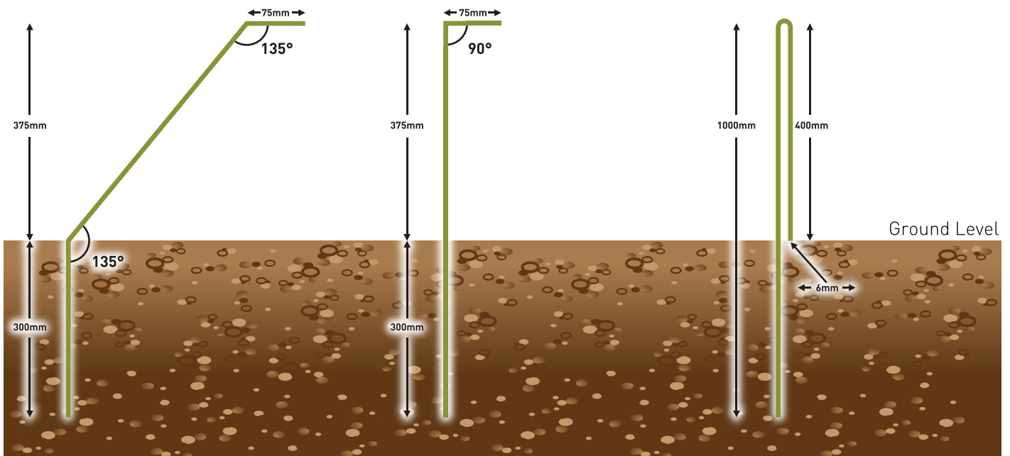
Profile of a one way TRAP panel
